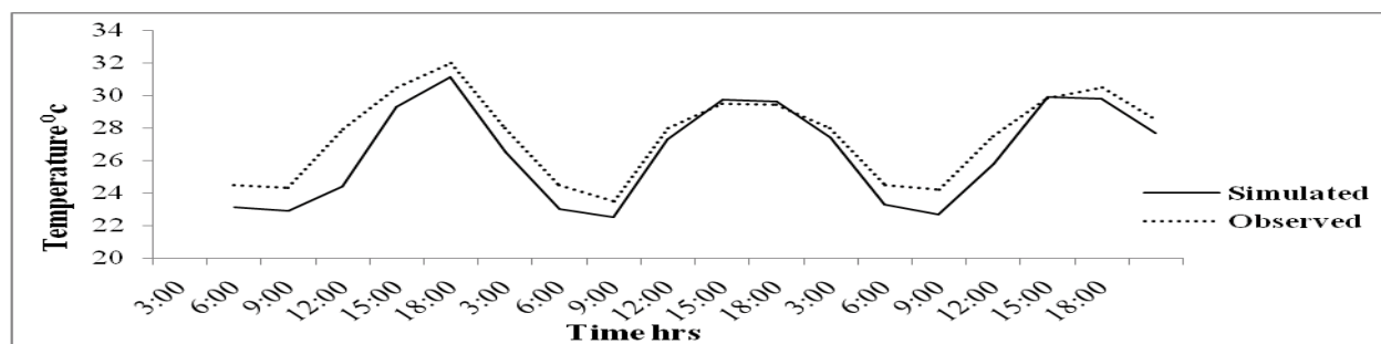
Figure 3: Diurnal patterns of simulated and observed (a) relative humidity; (b) wind speed; and (c) air temperature from 0600 UTC of 13 th to 2100 UTC of 15 th , December, 2012 over AKIA.
